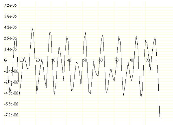
Figure 3. Evolution of the error function of the sequence leading to the maximal error
